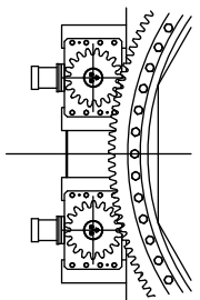
PINION ALIGNING DETAIL
