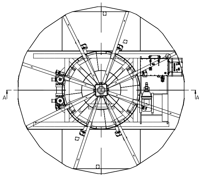
PINION ALIGNING DETAIL
